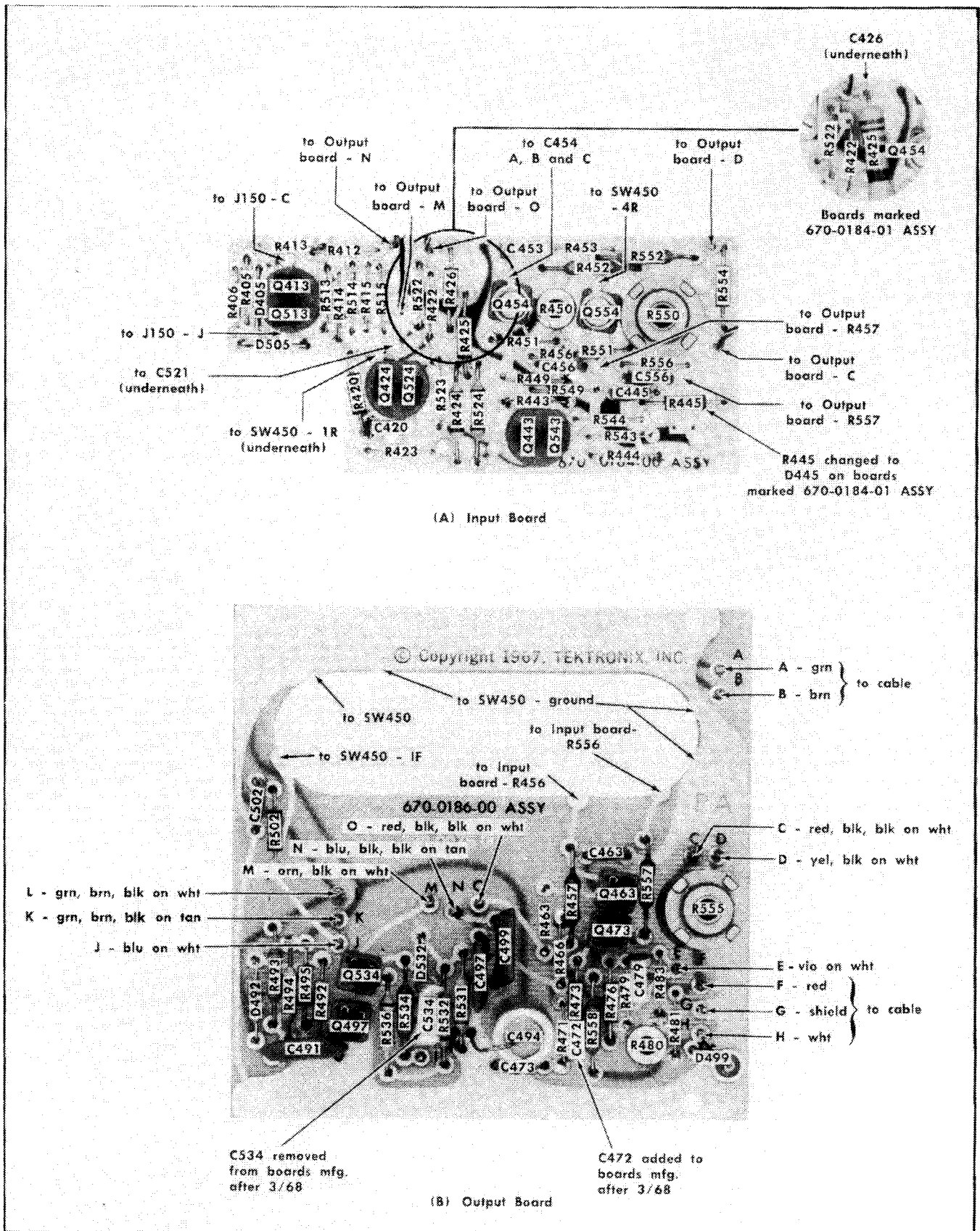
Fig. 6-4. Amplifier circuit board component locations.
